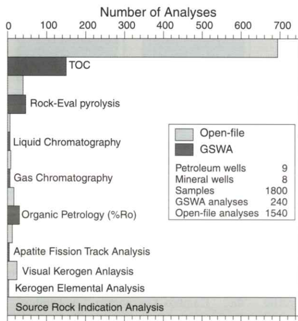
Figure 3: Project and open-file geochemical data used in this study.
