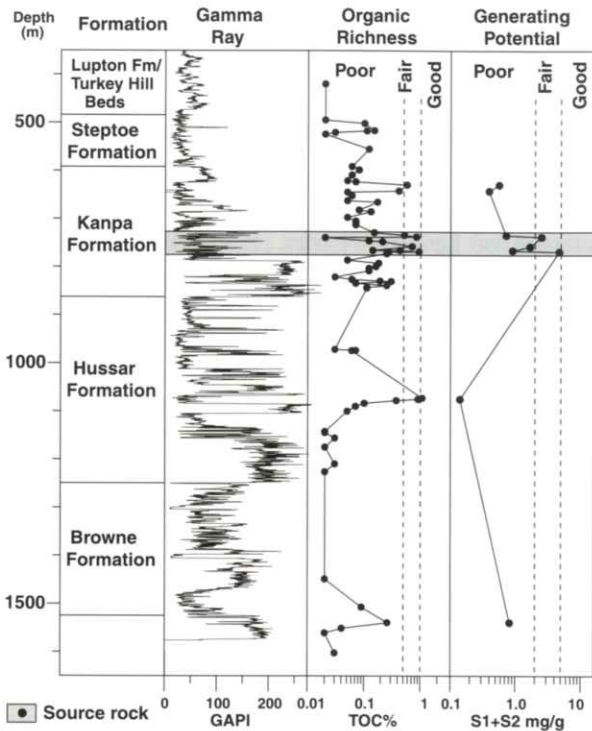
Figure 5: Organic richness and petroleum generating potential of rocks in Empress 1A.
