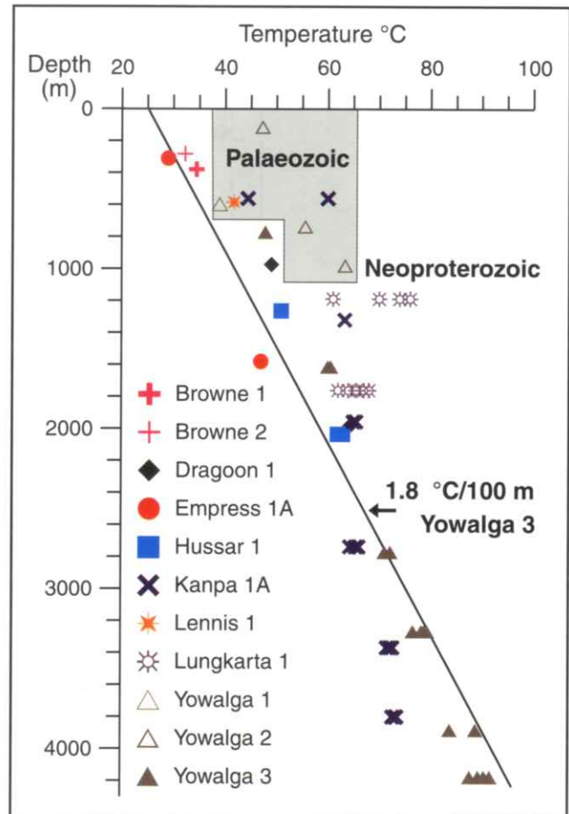
Figure 11: Present-day sub-surface temperature (BHT) versus depth.
