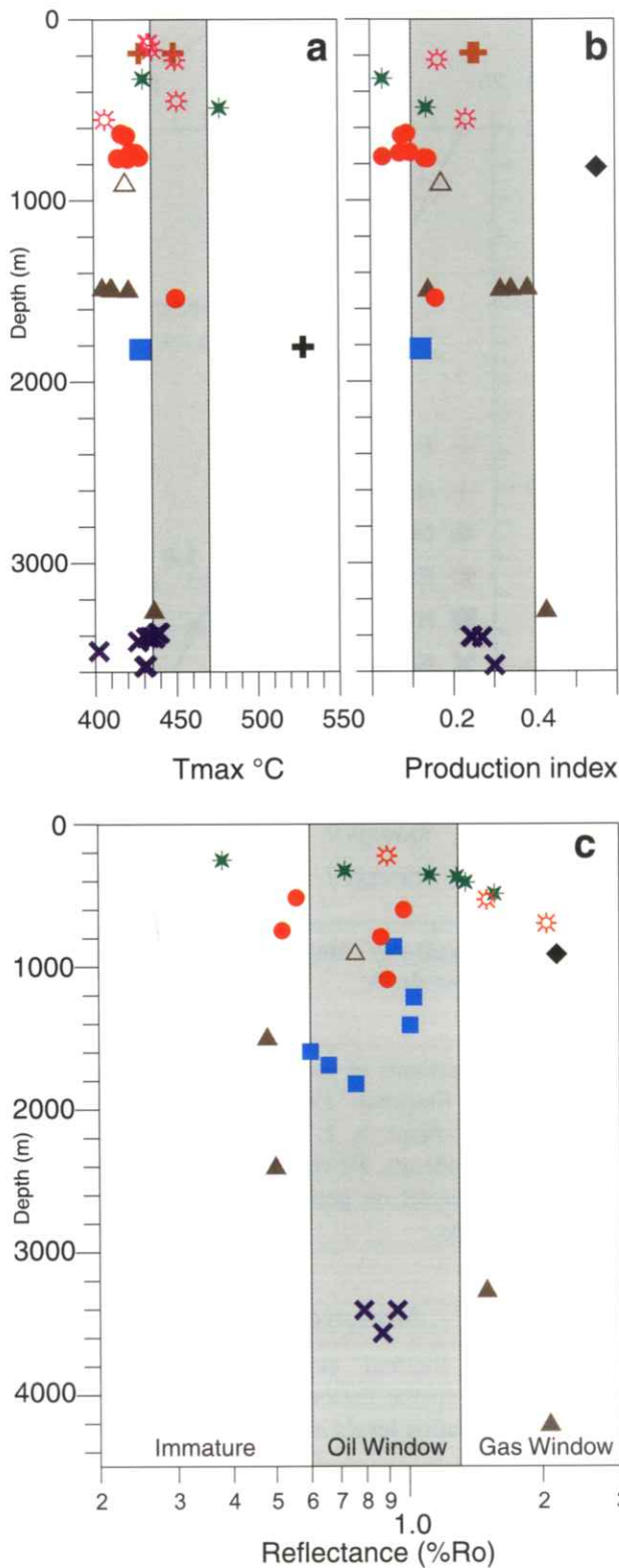
Figure 12: Measured maturity plots as depth versus: a) T_{max} ; b) Production Index; c) equivalent %Ro.
