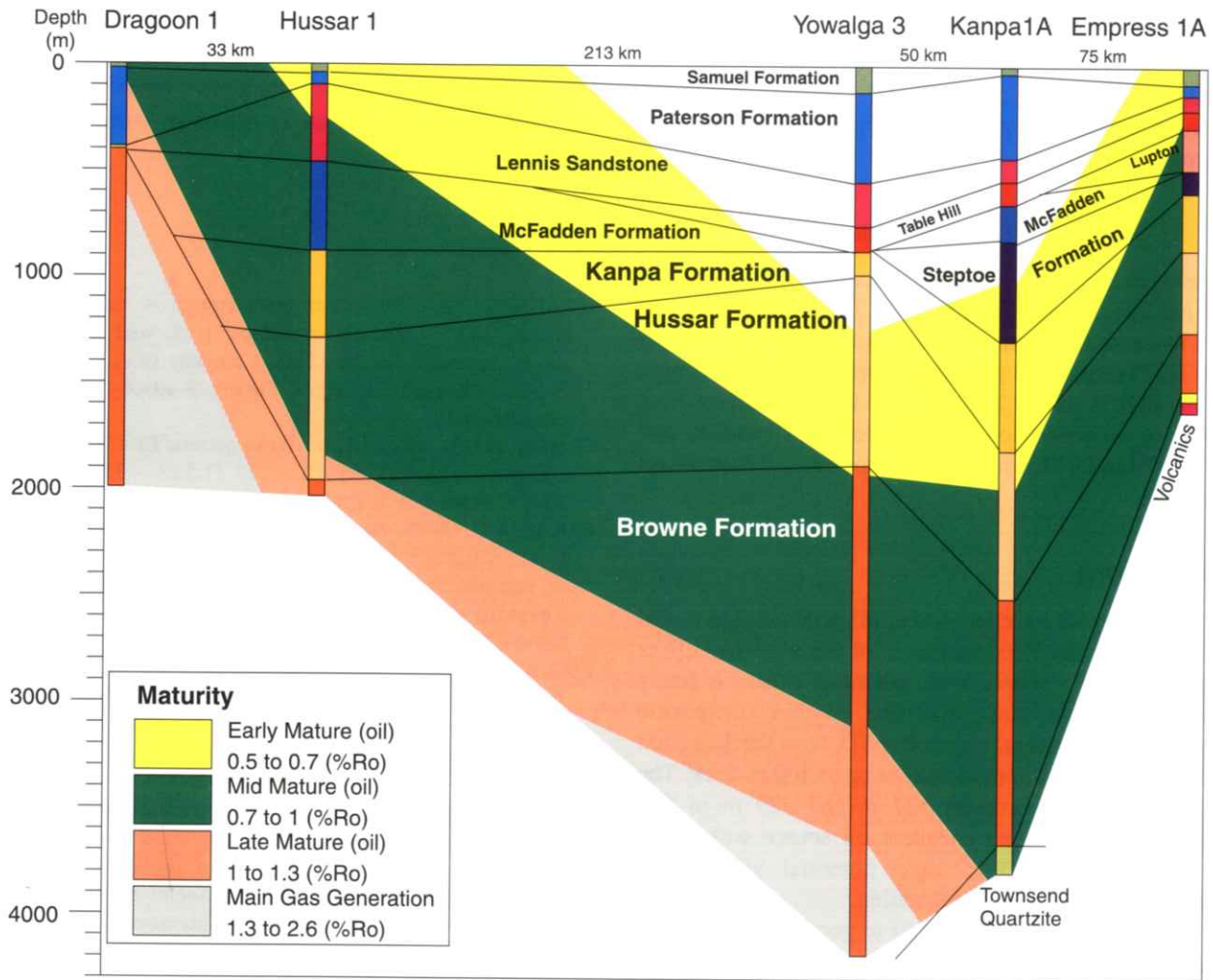
Figure 14: Neoproterozoic thermal maturity across the Yowalga and Gibson sub-basins from Dagoon 1 in the north to Empress 1A in the south. Well locations are shown in Figure 1.
