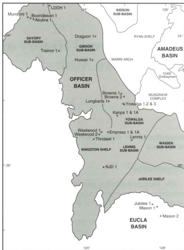
Figure 1: Location map of wells and sub-basins.
